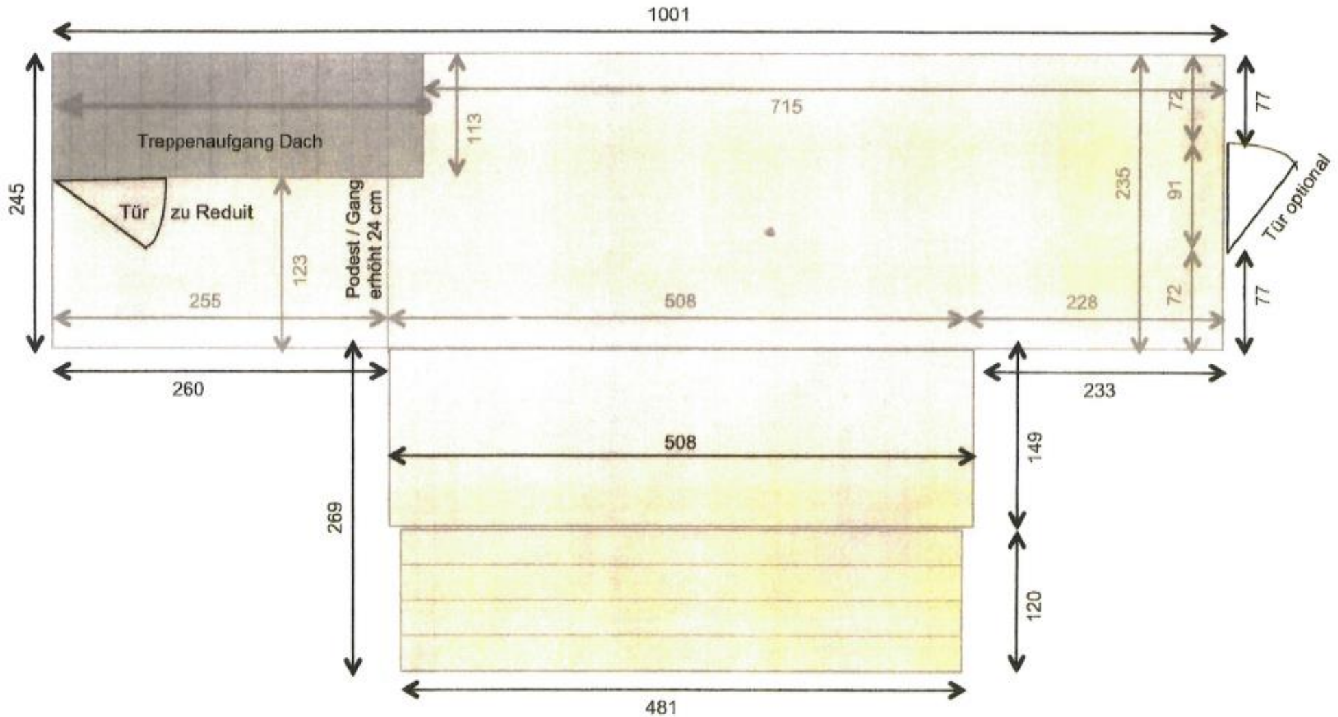
Detail Vermassung (in cm)
